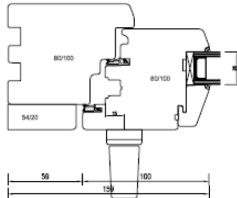
D. Side Section
