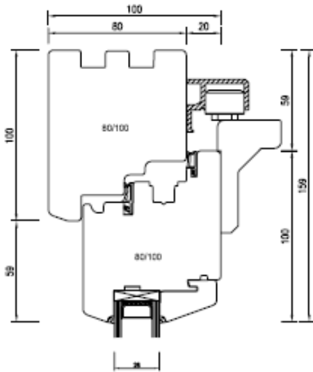
A. Head Section
