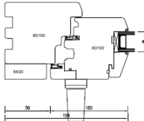
D. Side Section
