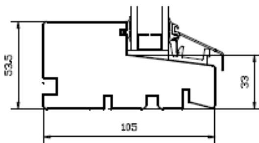
C. Sill Section
