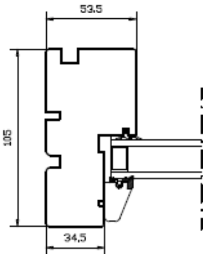
B. Side Section
